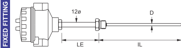
WITH FIXED FITTING AT A DISTANCE
