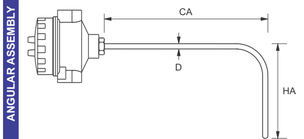
FACTORY BENT ASSEMBLY
