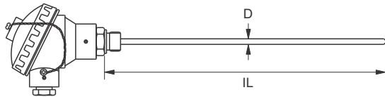
WITH HEX NIPPLE FIXED BELOW HEAD
