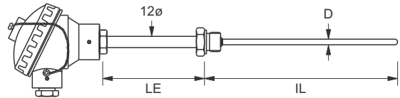
WITH FIXED FITTING AT A DISTANCE
